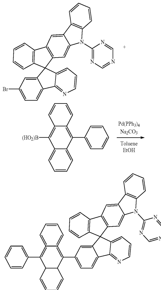
Compound 9
