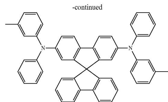
Spiro-TPD
